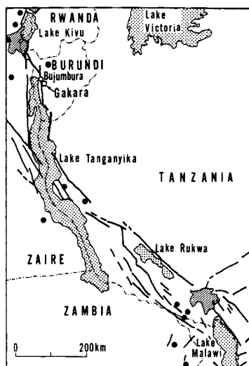
Fig. 1. Location of the Gakara REE deposits and the Western Rift in Central Africa, with faults (thick lines). Shaded parts and solid circles indicate Cenozoic volcanic provinces and Late Proterozoic alkaline massifs, respectively.
