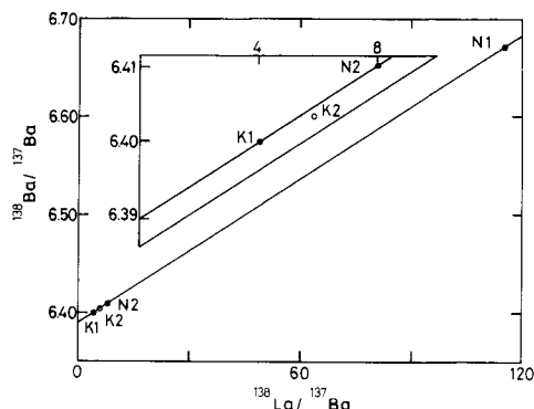
Fig. 2. La-Ba mineral-isochron plot for the Gakara bastnaesite-monzazite deposits, Burundi. The isochron line except for K2 yields an age of 586.8 \pm 3.7 Ma ( 2\sigma_m ) ( \lambda_{\text{EC}} = 4.15 \times 10^{-12} yr ^{-1} ) with an initial ^{138}\text{Ba}/^{137}\text{Ba} ratio of 6.39005 \pm 0.00030 ( 2\sigma_m ).
